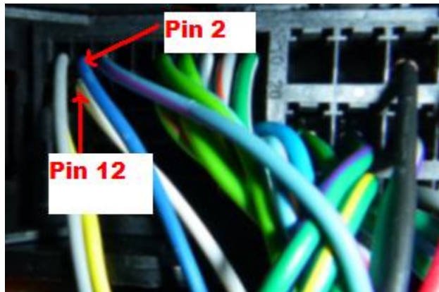
This is the view of the connector in the vehicle
