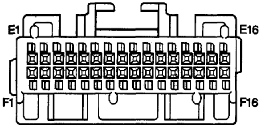
This is the pin view of the connector in the vehicle
