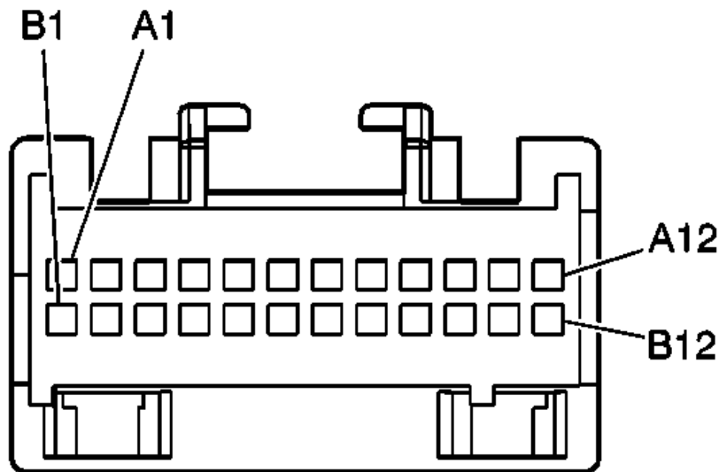
This is the pin view of the connector in the vehicle
